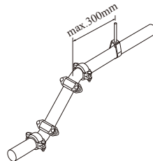
Short riser (or short drop)
