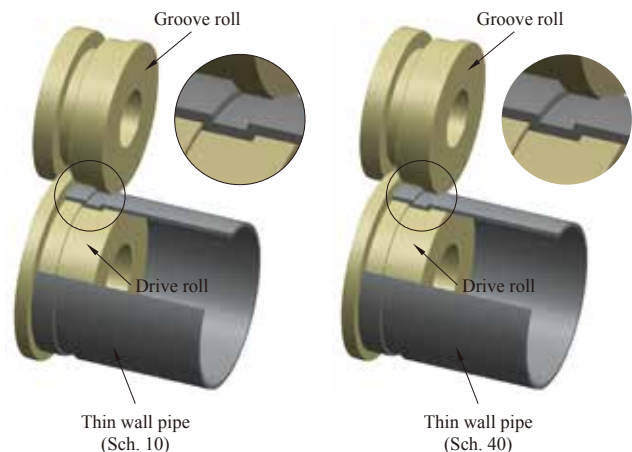
Different roll set (Groove & Drive roll) W2 should be wider than W1
