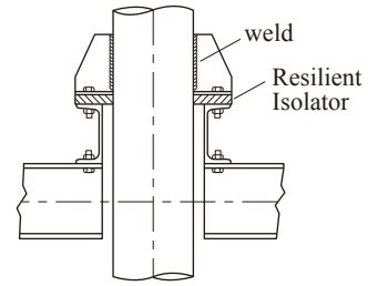
Anchors for risers ( ➔➔ )
